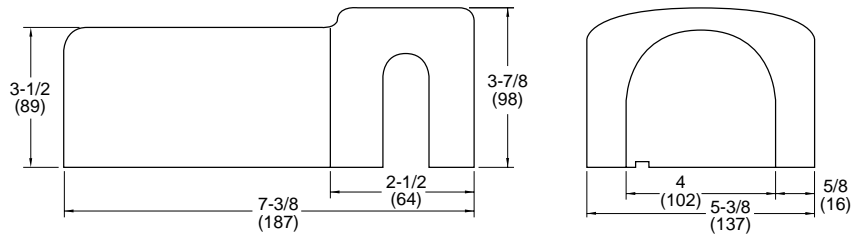
MOTOR COVER
